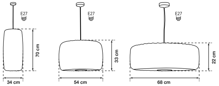
PLANET WHITE POLYMER CYLINDER PENDANT 68cm H1C2YRBJRSC-068
