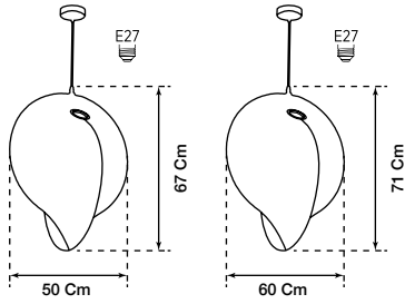
Product Dimensions and Socket Type
